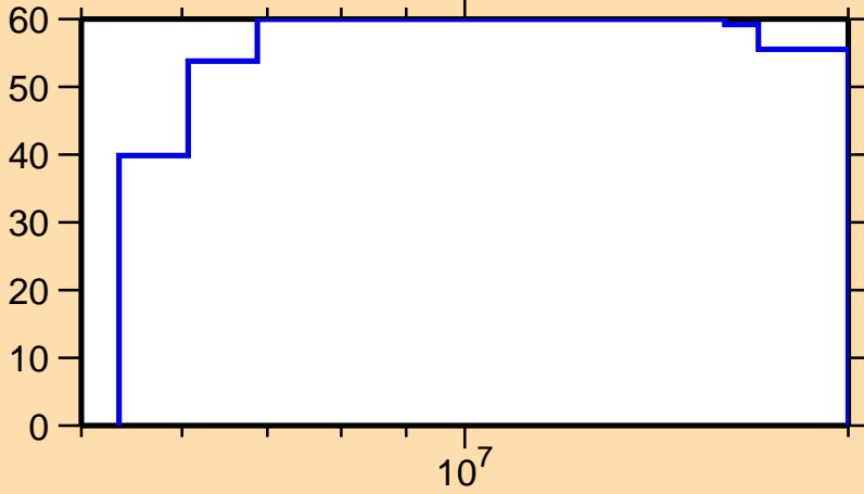
\Delta\sigma/\sigma vs. E for ^{230}\text{Pa}(n,2n)
