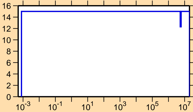
\Delta v/v vs. E for ^{230}\text{Pa} (delayed \nu )
