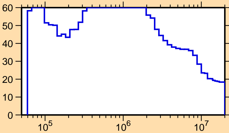
\Delta\sigma/\sigma vs. E for ^{230}\text{Pa}(n,\text{inel.})
