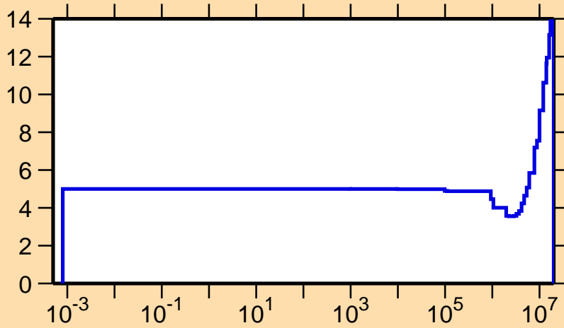
\Delta v/v vs. E for ^{230}\text{Pa} (prompt \nu )
