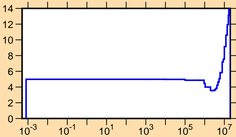
\Delta v/v vs. E for ^{230}\text{Pa} (total v )
