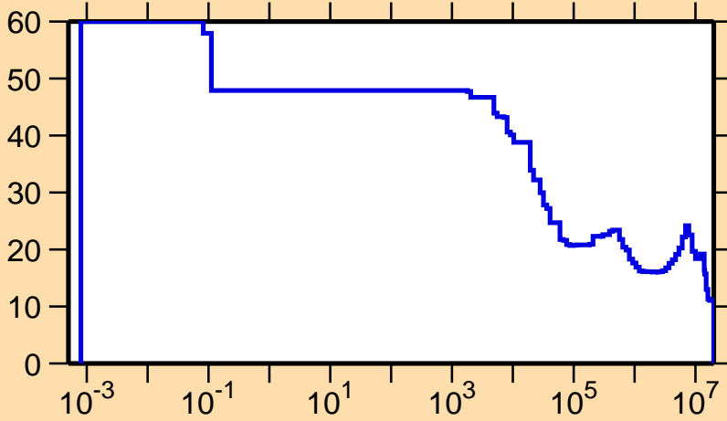
\Delta\sigma/\sigma vs. E for ^{230}\text{Pa}(n,f)
