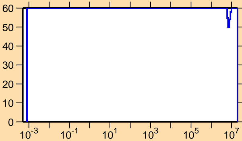
\Delta\sigma/\sigma vs. E for ^{230}\text{Pa}(n,\gamma)
