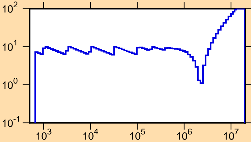
\Delta\phi/\phi vs. E for ^{230}\text{Pa}(n,f)
