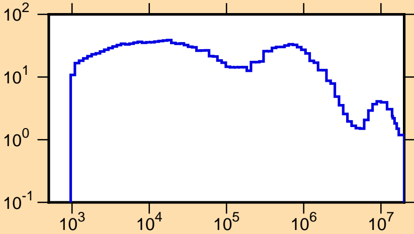
\Delta\mu/\mu vs. E for ^{230}\text{Pa}(\text{mt251})
