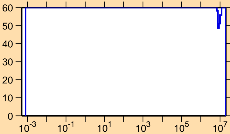
\Delta\sigma/\sigma vs. E for ^{229}\text{Pa}(n,\gamma)
