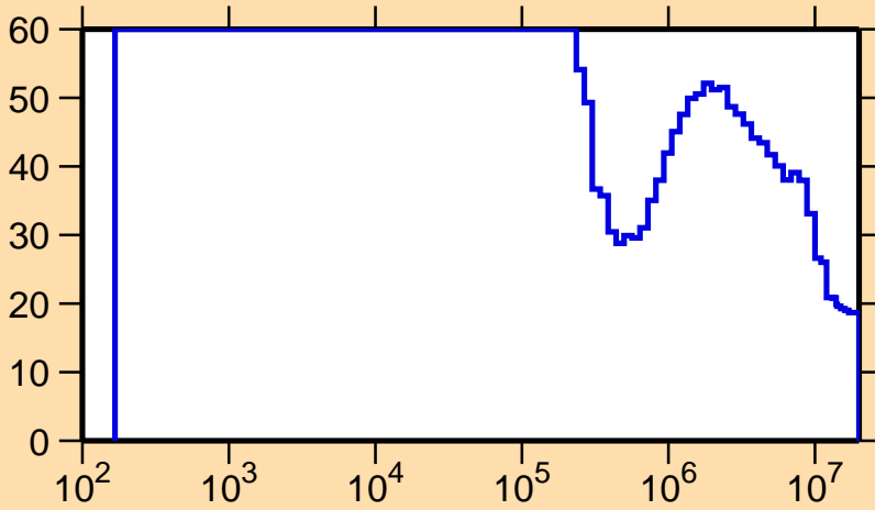
\Delta\sigma/\sigma vs. E for ^{229}\text{Pa}(n,\text{inel.})
