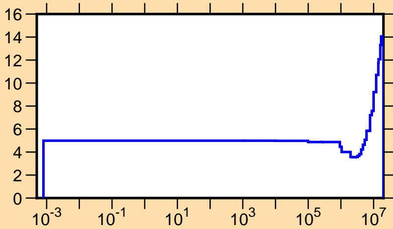
\Delta v/v vs. E for ^{229}\text{Pa}(\text{total } \nu)
