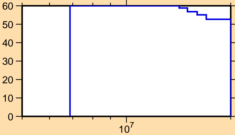
\Delta\sigma/\sigma vs. E for ^{229}\text{Pa}(n,2n)
