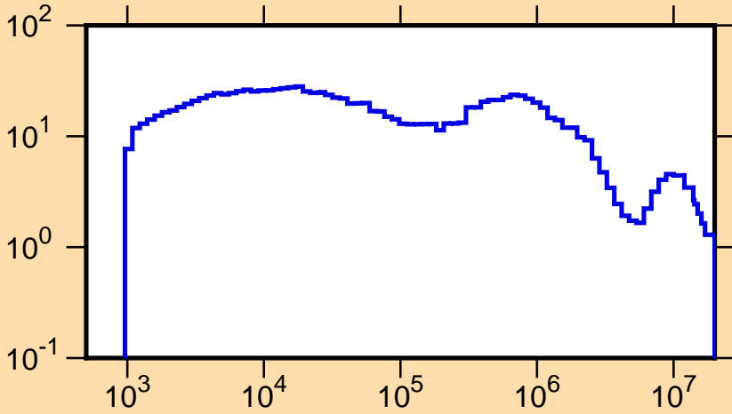
\Delta\mu/\mu vs. E for ^{229}\text{Pa}(\text{mt251})
