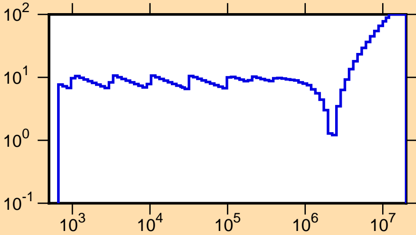
\Delta\phi/\phi vs. E for ^{229}\text{Pa}(n,f)
