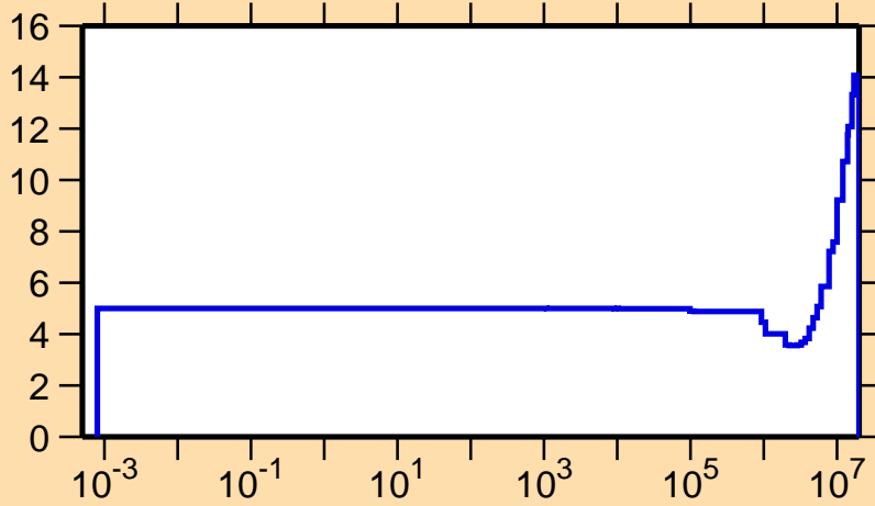
\Delta v/v vs. E for ^{229}\text{Pa} (prompt \nu )
