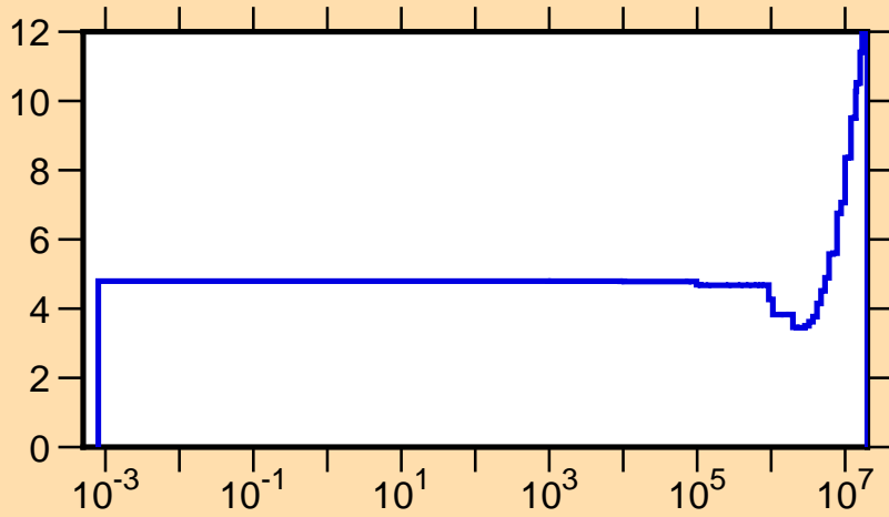
\Delta v/v vs. E for ^{234}\text{Th}(\text{total } \nu)
