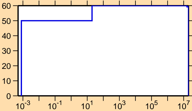
\Delta\sigma/\sigma vs. E for ^{234}\text{Th}(n,f)
