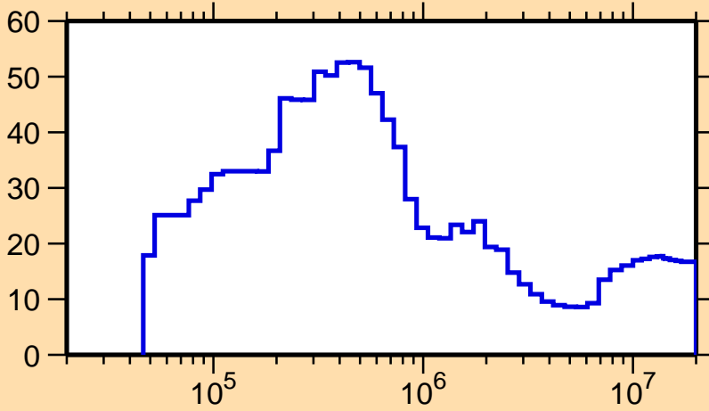
\Delta\sigma/\sigma vs. E for ^{234}\text{Th}(n,\text{inel.})
