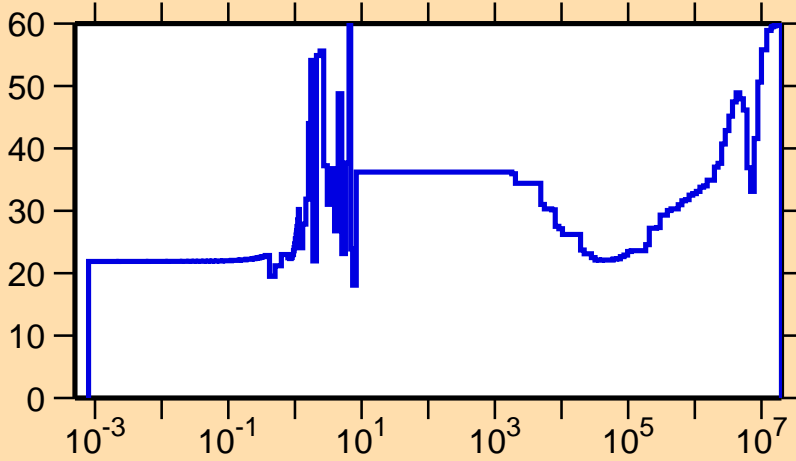
\Delta\sigma/\sigma vs. E for ^{229}\text{Th}(n,\gamma)
