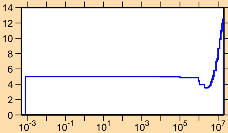
\Delta v/v vs. E for ^{229}\text{Th}(\text{prompt } \nu)
