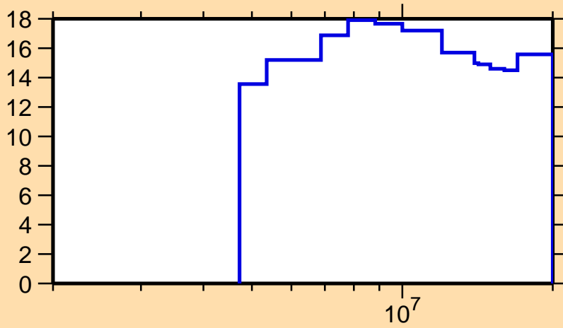
\Delta\sigma/\sigma vs. E for ^{229}\text{Th}(n,2n)
