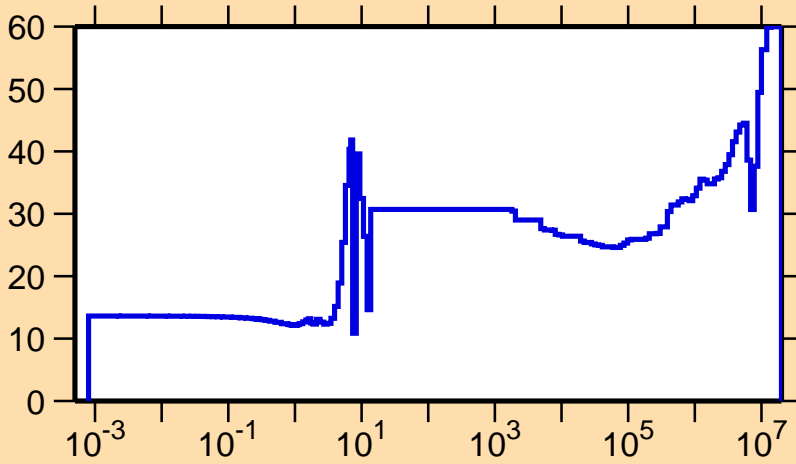
\Delta\sigma/\sigma vs. E for ^{228}\text{Th}(n,\gamma)
