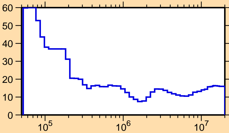
\Delta\sigma/\sigma vs. E for ^{228}\text{Th}(n,\text{inel.})
