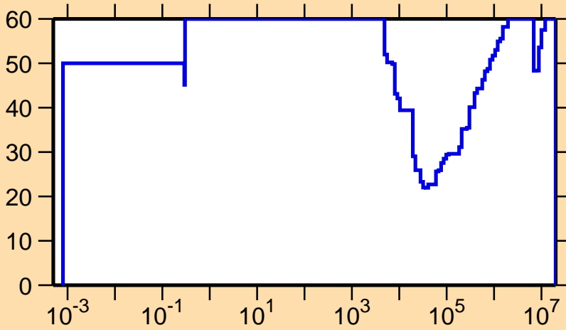
\Delta\sigma/\sigma vs. E for ^{226}\text{Ac}(n,\gamma)
