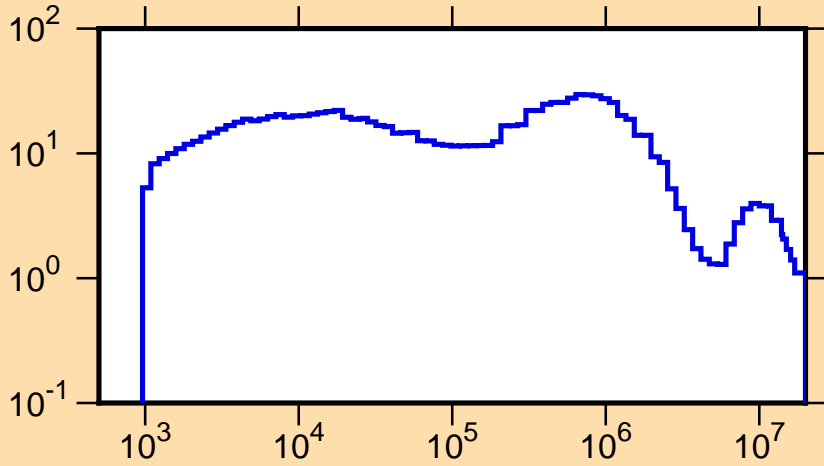
\Delta\mu/\mu vs. E for ^{226}\text{Ac}(\text{mt251})
