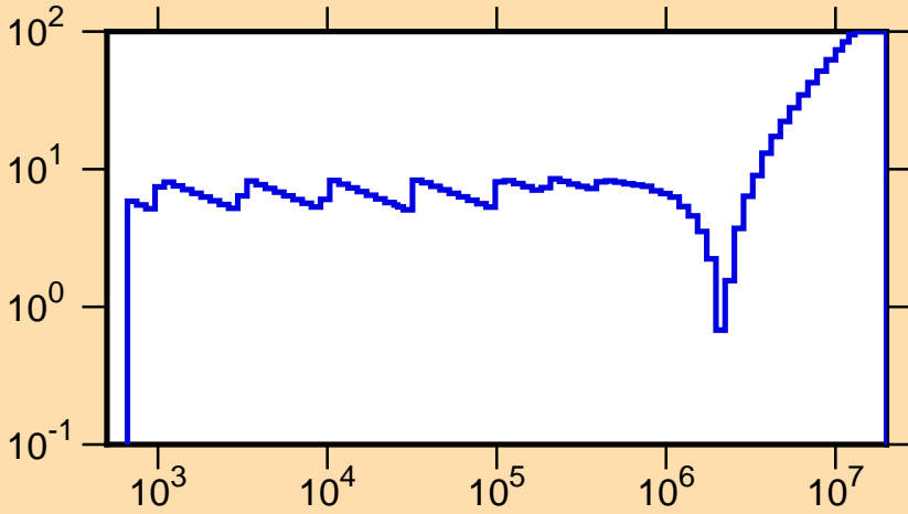
\Delta\phi/\phi vs. E for ^{226}\text{Ac}(n,f)
