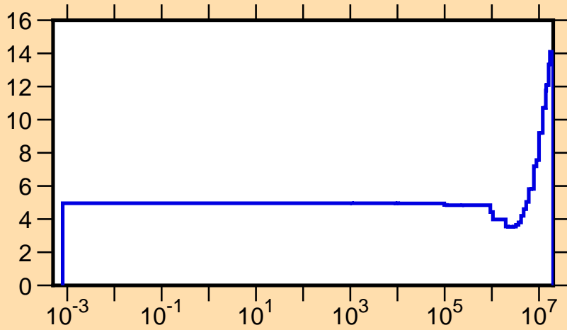
\Delta v/v vs. E for ^{226}\text{Ac}(\text{total } \nu)
