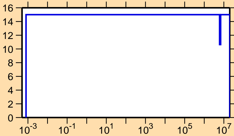
\Delta\nu/\nu vs. E for ^{226}\text{Ac}(\text{delayed } \nu)
