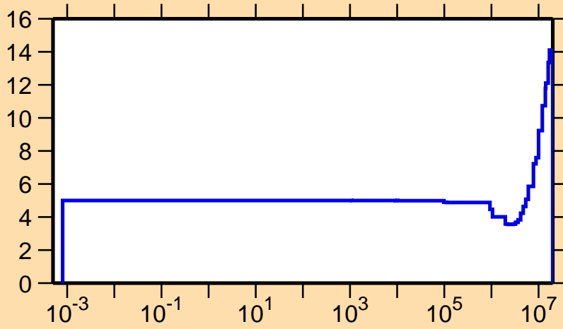
\Delta v/v vs. E for ^{226}\text{Ac} (prompt \nu )
