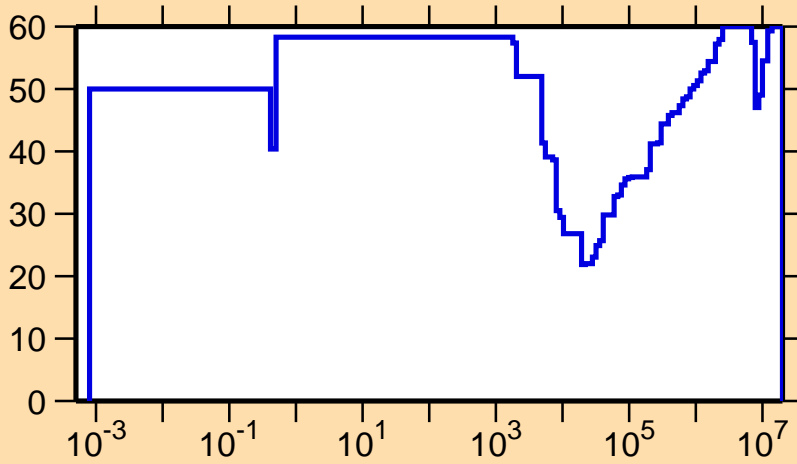
\Delta\sigma/\sigma vs. E for ^{225}\text{Ac}(n,\gamma)
