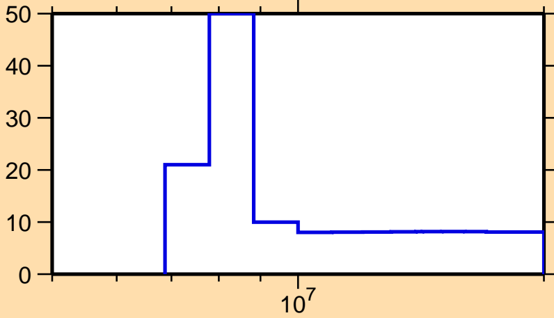
\Delta\sigma/\sigma vs. E for ^{208}\text{Pb}(n,2n)
