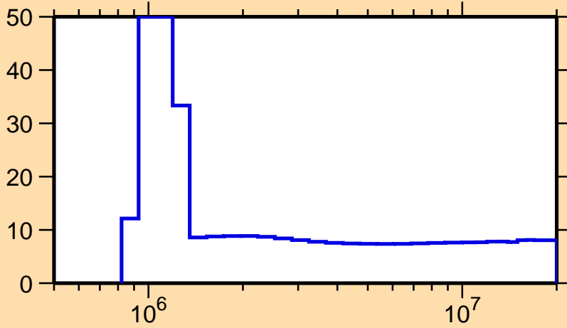
\Delta\sigma/\sigma vs. E for ^{204}\text{Pb}(n,\text{inel.})
