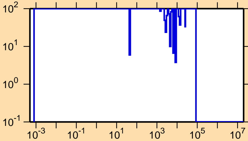
\Delta\sigma/\sigma vs. E for ^{205}\text{Tl}(n,\gamma)
