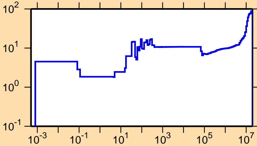
\Delta\sigma/\sigma vs. E for ^{193}\text{Ir}(n,\gamma)
