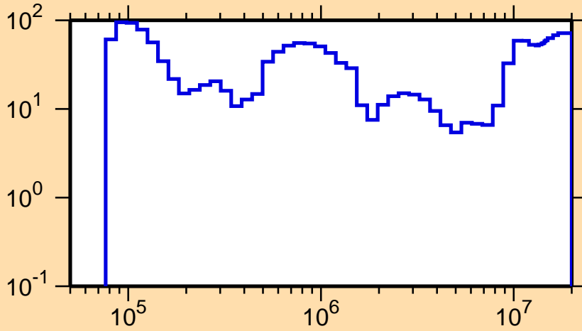
\Delta\sigma/\sigma vs. E for ^{193}\text{Ir}(n,\text{inel.})
