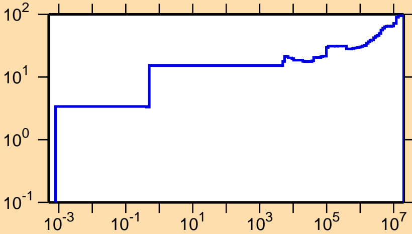
\Delta\sigma/\sigma vs. E for ^{170}\text{Er}(n,\gamma)
