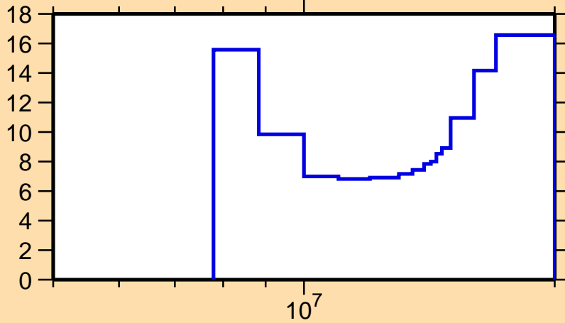
\Delta\sigma/\sigma vs. E for ^{158}\text{Gd}(n,2n)
