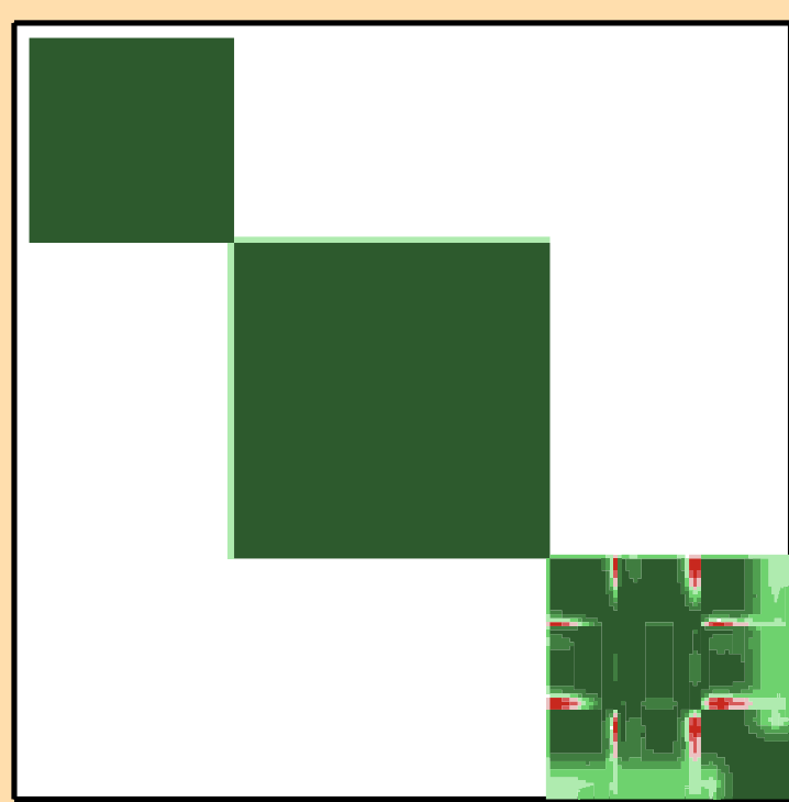
Correlation Matrix
