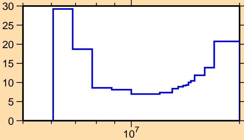
\Delta\sigma/\sigma vs. E for ^{157}\text{Gd}(n,2n)
