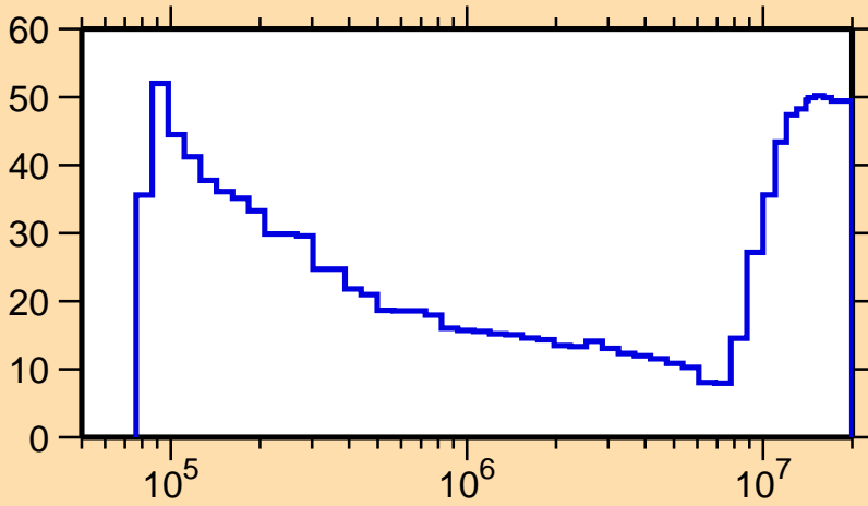
\Delta\sigma/\sigma vs. E for ^{155}\text{Gd}(n,\text{inel.})
