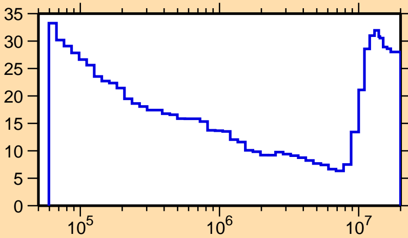
\Delta\sigma/\sigma vs. E for ^{153}\text{Gd}(n,\text{inel.})
