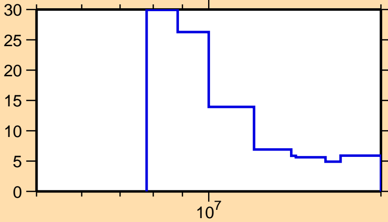
\Delta\sigma/\sigma vs. E for ^{155}\text{Eu}(n,2n)
