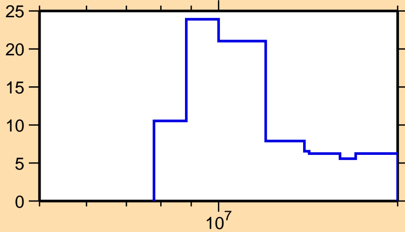
\Delta\sigma/\sigma vs. E for ^{153}\text{Eu}(n,2n)
