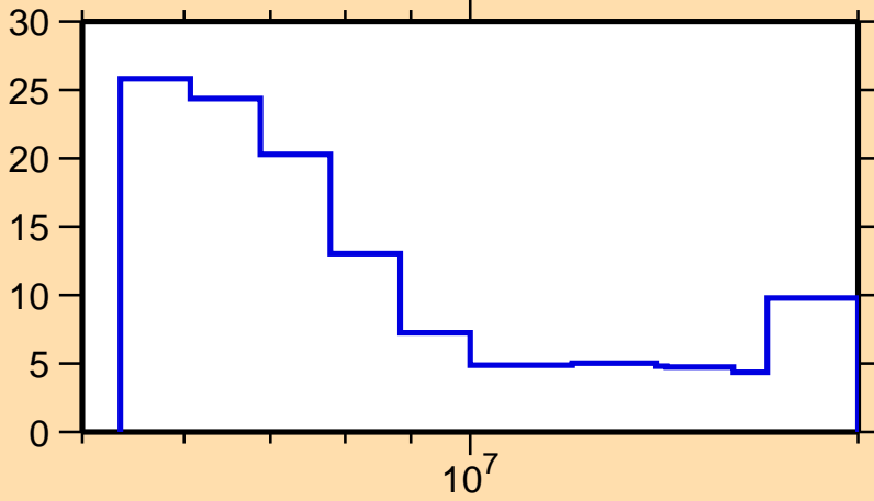
\Delta\sigma/\sigma vs. E for ^{151}\text{Sm}(n,2n)
