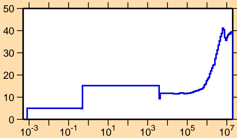
\Delta\sigma/\sigma vs. E for ^{145}\text{Nd}(n,\gamma)
