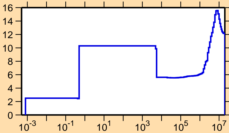
\Delta\sigma/\sigma vs. E for ^{143}\text{Nd}(n,\text{el.})
