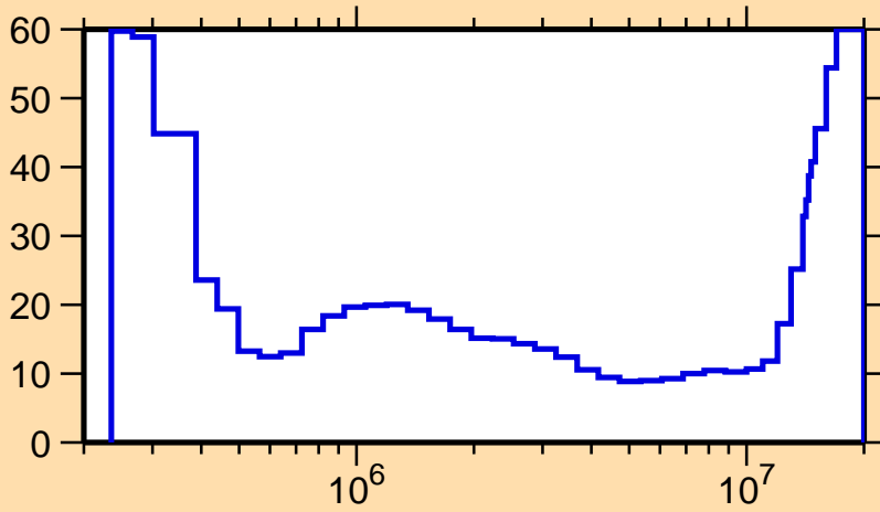
\Delta\sigma/\sigma vs. E for ^{135}\text{Cs}(n,\text{inel.})
