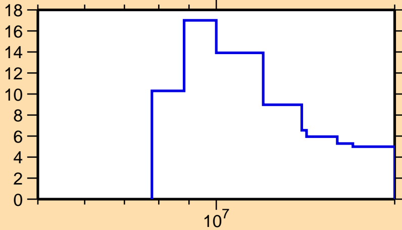
\Delta\sigma/\sigma vs. E for ^{134}\text{Xe}(n,2n)
