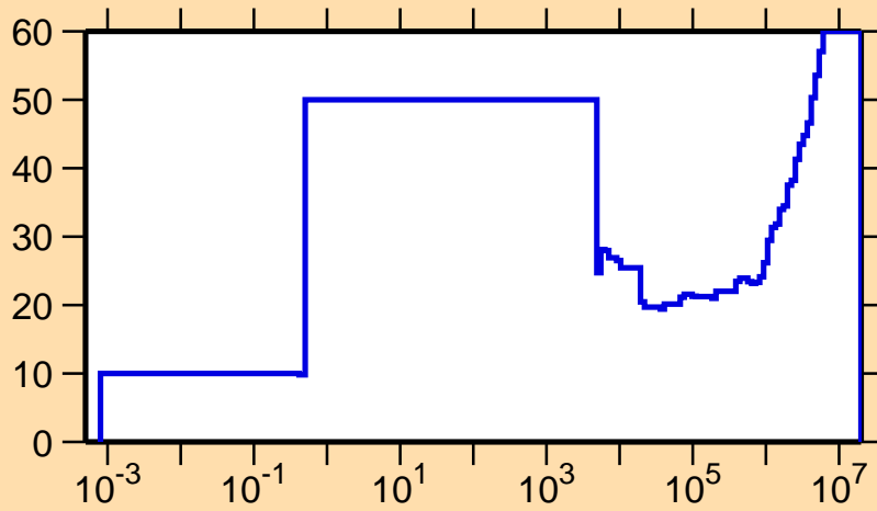
\Delta\sigma/\sigma vs. E for ^{134}\text{Xe}(n,\gamma)
