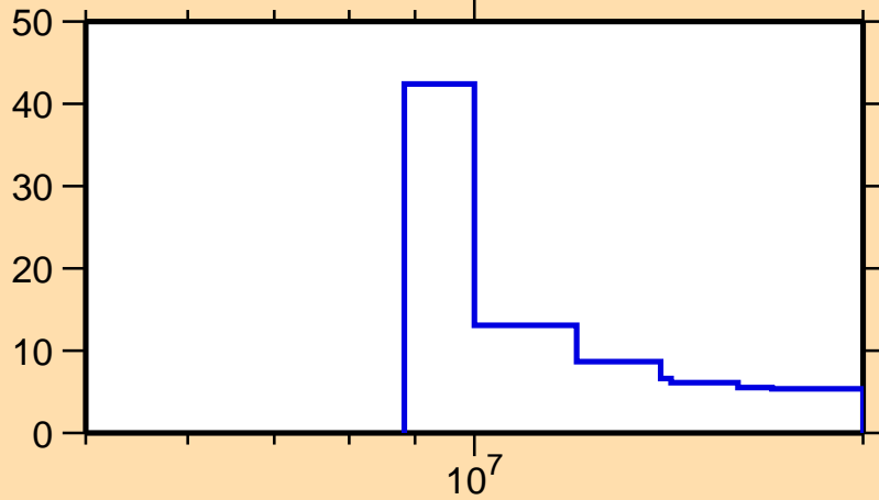
\Delta\sigma/\sigma vs. E for ^{132}\text{Xe}(n,2n)
