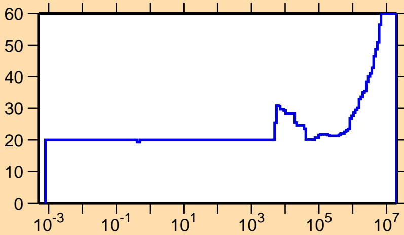
\Delta\sigma/\sigma vs. E for ^{132}\text{Xe}(n,\gamma)
