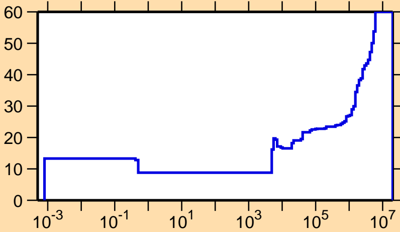
\Delta\sigma/\sigma vs. E for ^{129}\text{I}(n,\gamma)
