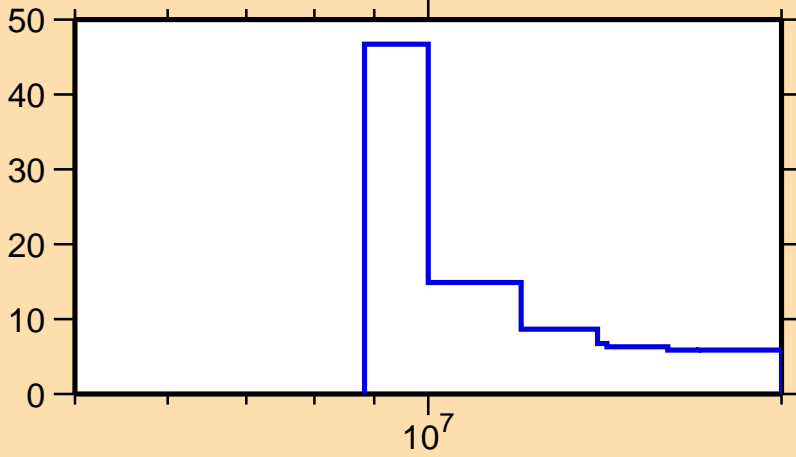
\Delta\sigma/\sigma vs. E for ^{129}\text{I}(n,2n)
