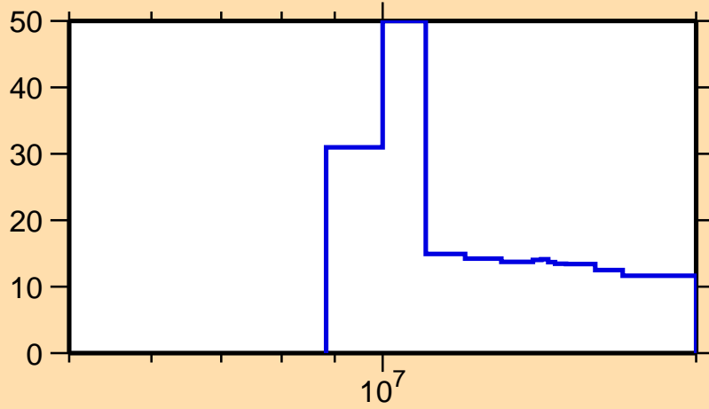
\Delta\sigma/\sigma vs. E for ^{109}\text{Ag}(n,2n)
