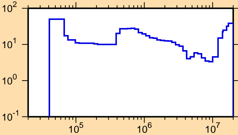
\Delta\sigma/\sigma vs. E for ^{103}\text{Rh}(n,\text{inel.})
