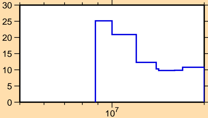
\Delta\sigma/\sigma vs. E for ^{103}\text{Rh}(n,2n)
