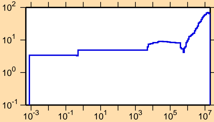
\Delta\sigma/\sigma vs. E for ^{103}\text{Rh}(n,\gamma)
