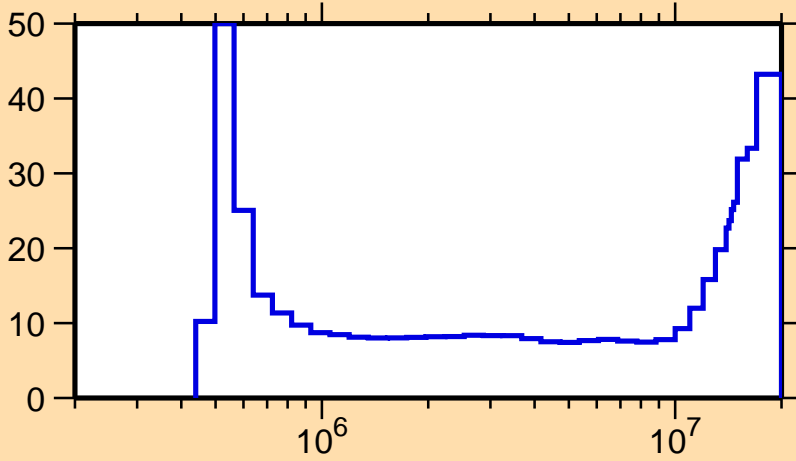
\Delta\sigma/\sigma vs. E for ^{97}\text{Mo}(n,\text{inel.})
