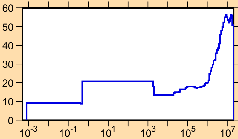
\Delta\sigma/\sigma vs. E for ^{97}\text{Mo}(n,\gamma)
