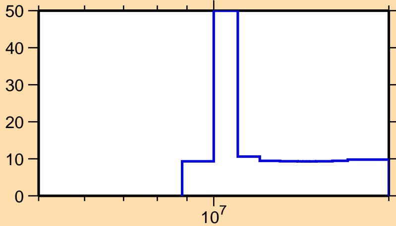
\Delta\sigma/\sigma vs. E for ^{94}\text{Mo}(n,2n)
