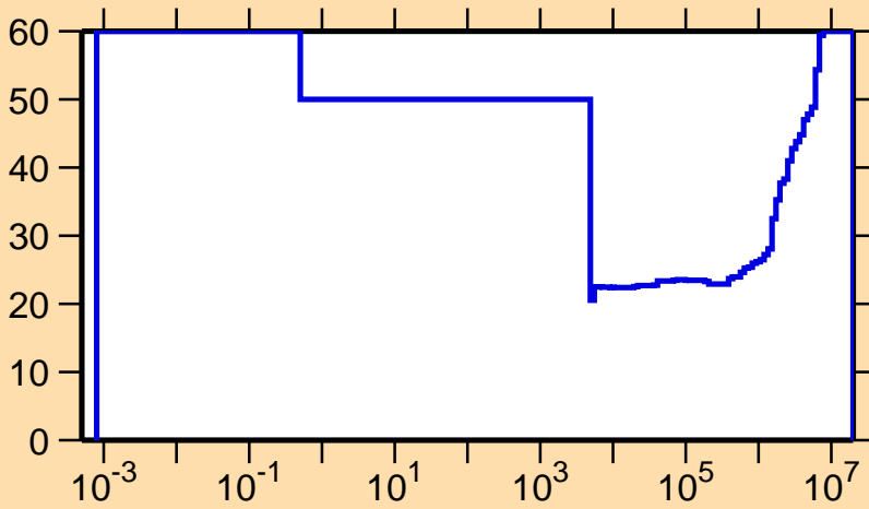
\Delta\sigma/\sigma vs. E for ^{95}\text{Nb}(n,\gamma)
