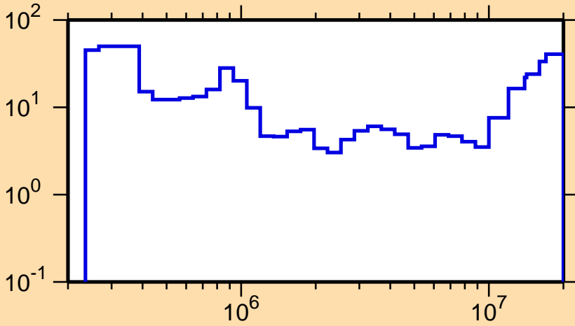
\Delta\sigma/\sigma vs. E for ^{95}\text{Nb}(n,\text{inel.})
