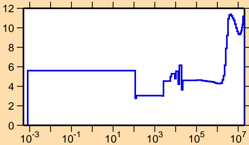
\Delta\sigma/\sigma vs. E for ^{91}\text{Zr}(n,\text{el.})
