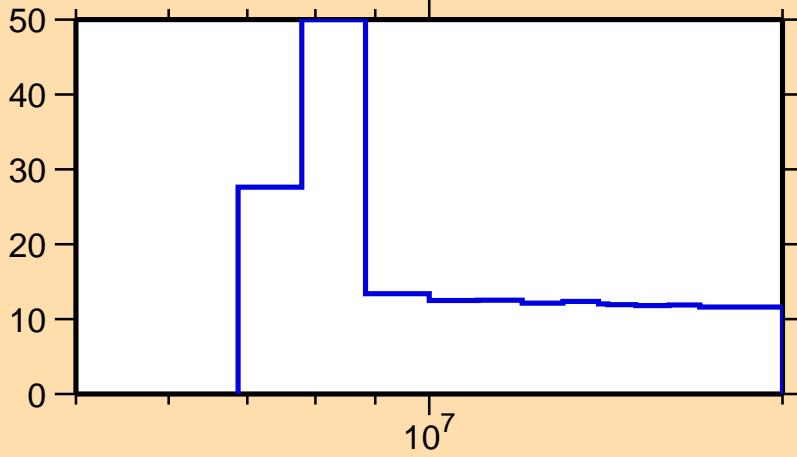
\Delta\sigma/\sigma vs. E for ^{91}\text{Zr}(n,2n)
