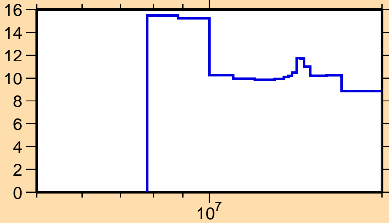
\Delta\sigma/\sigma vs. E for ^{53}\text{Cr}(n,2n)
