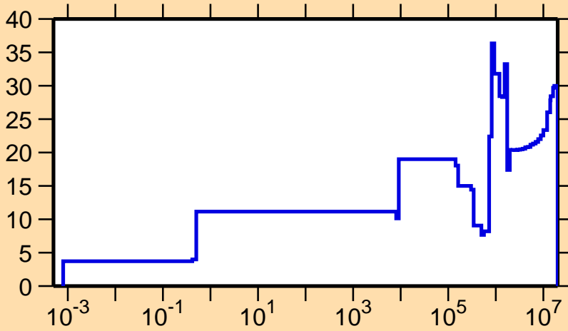
\Delta\sigma/\sigma vs. E for ^{24}\text{Mg}(n,\gamma)
