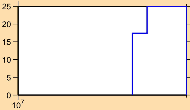
\Delta\sigma/\sigma vs. E for ^{16}\text{O}(n,2n)
