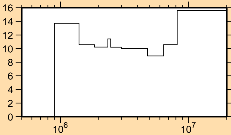
\Delta\sigma/\sigma vs. E for ^{57}\text{Fe}(n,n_5)
