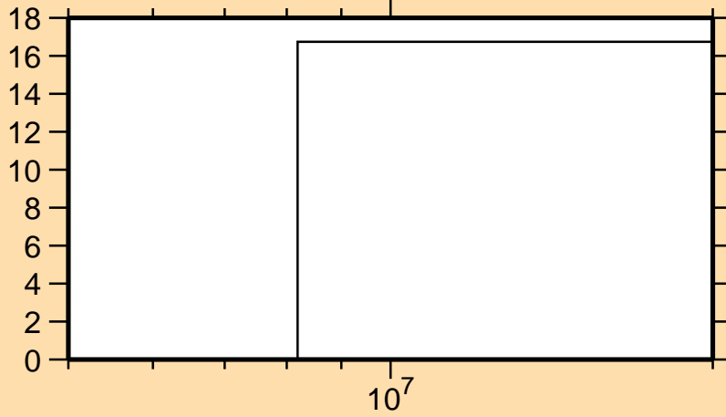
\Delta\sigma/\sigma vs. E for ^{57}\text{Fe}(n,np)
