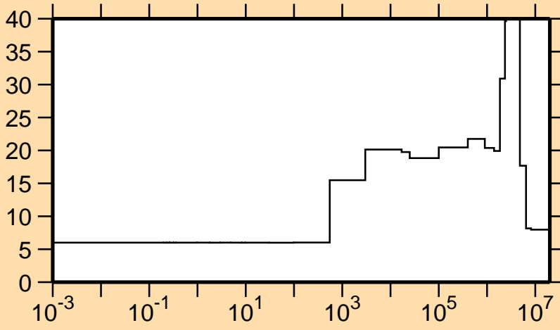
\Delta\sigma/\sigma vs. E for C(n,nonel.)
