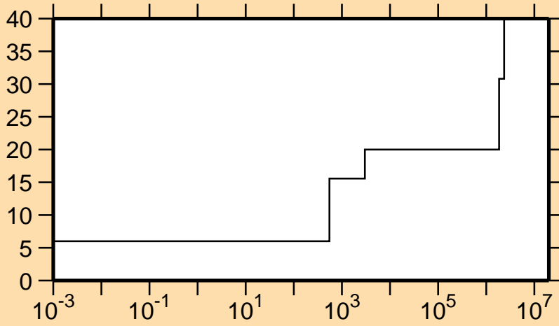
\Delta\sigma/\sigma vs. E for C(n, \gamma )
