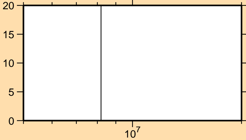
\Delta\sigma/\sigma vs. E for C(n,p)
