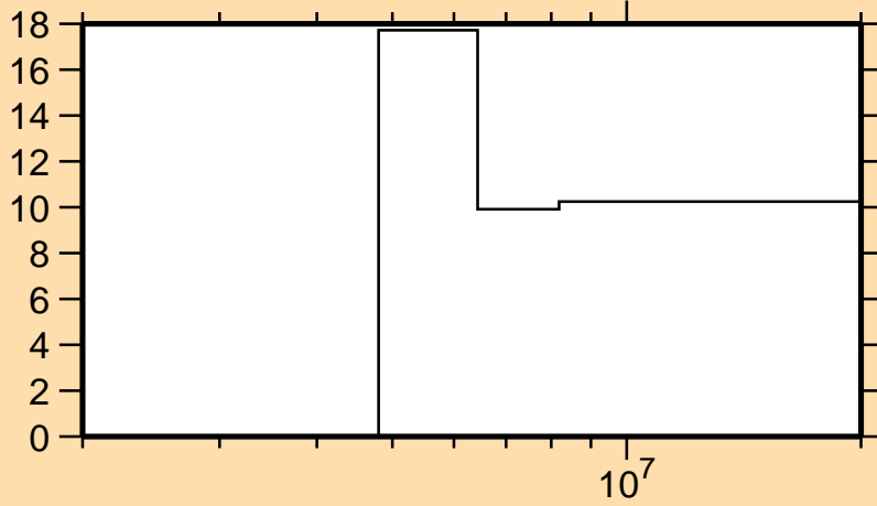
\Delta\sigma/\sigma vs. E for C(n,incl.)
