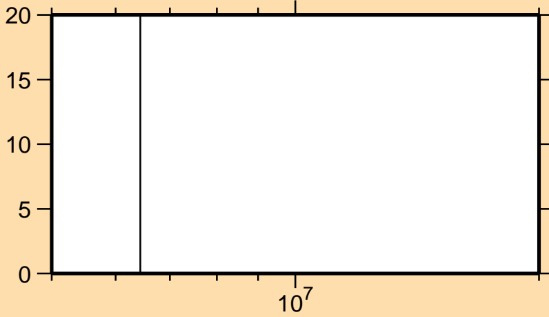
\Delta\sigma/\sigma vs. E for C(n,ncont.)
