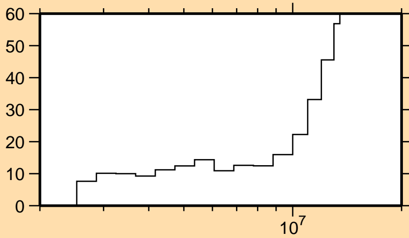
\Delta\sigma/\sigma vs. E for ^{54}\text{Fe}(n,n_3)
