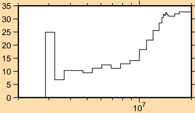
\Delta\sigma/\sigma vs. E for ^{54}\text{Fe}(n,n_6)
