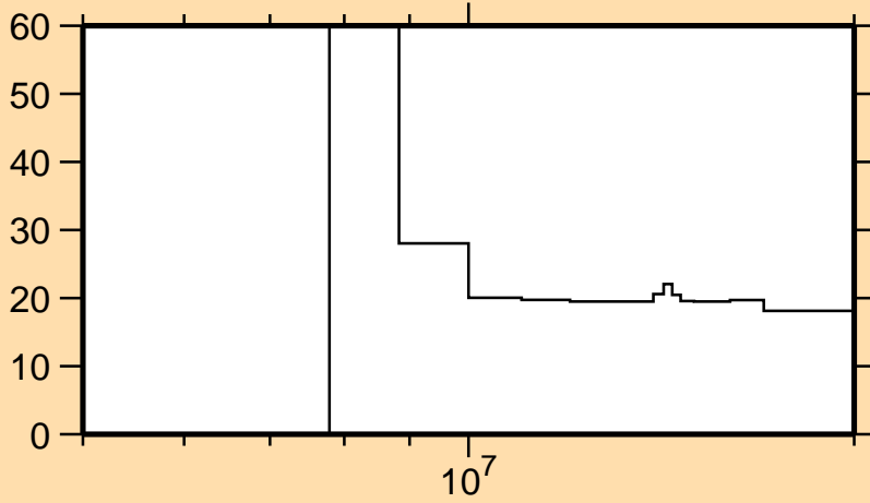
\Delta\sigma/\sigma vs. E for ^{54}\text{Fe}(n,n\alpha)
