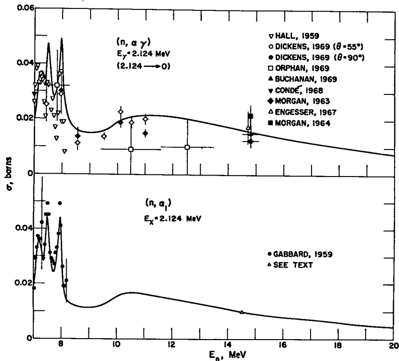
Fig. 60. Measured and evaluated (n, \alpha_1) and (n, \alpha \gamma) cross sections for the 2.124-MeV level and ground-state transition. The 14.5-MeV (n, \alpha_1) datum is a composite of four measurements.
