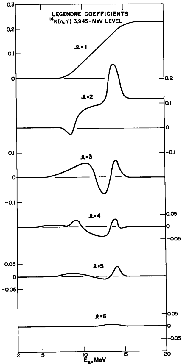
Fig. C3. Evaluated Legendre coefficients for inelastic scattering to the 3.945-MeV level in 14 N. This transition exhibits the largest l=2 coefficient of any inelastic channel for nitrogen.
