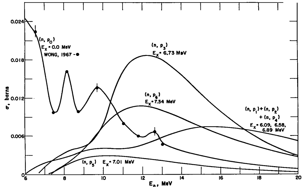
Fig. 44. Evaluated cross sections from 6 to 20 MeV for the (n, p) reaction to the six particle-stable excited states in ^{14}\text{C} , together with the (n, p_0) cross section and the data on which it is based.
