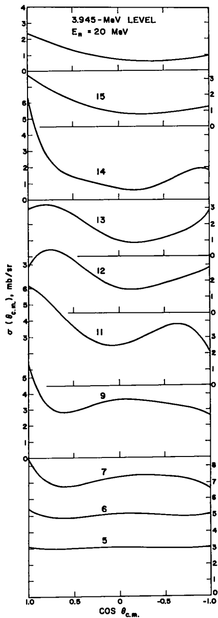
Fig. C4. Evaluated differential cross sections at selected energies for inelastic scattering to the 3.945-MeV level in 14 N.
