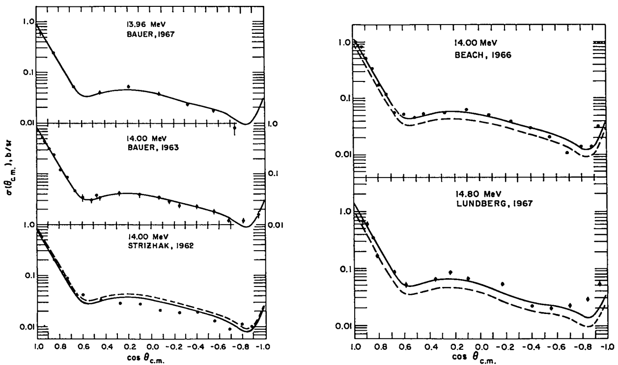
Fig. 83. Measured and evaluated differential cross sections for elastic scattering from 13.9 to 14.8 MeV.
