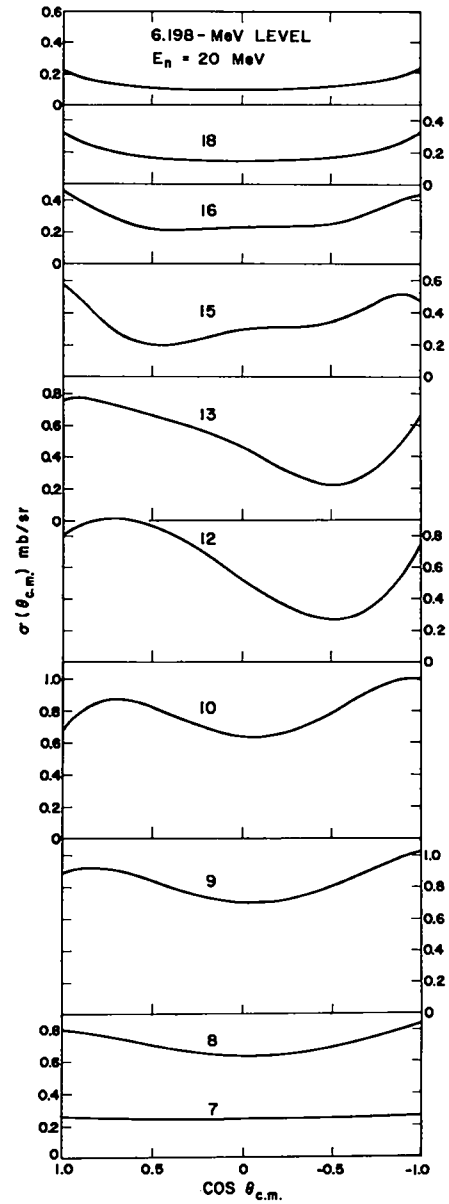
Fig. C14. Evaluated differential cross sections at selected energies for inelastic scattering to the 6.198-MeV level in 14 N.
