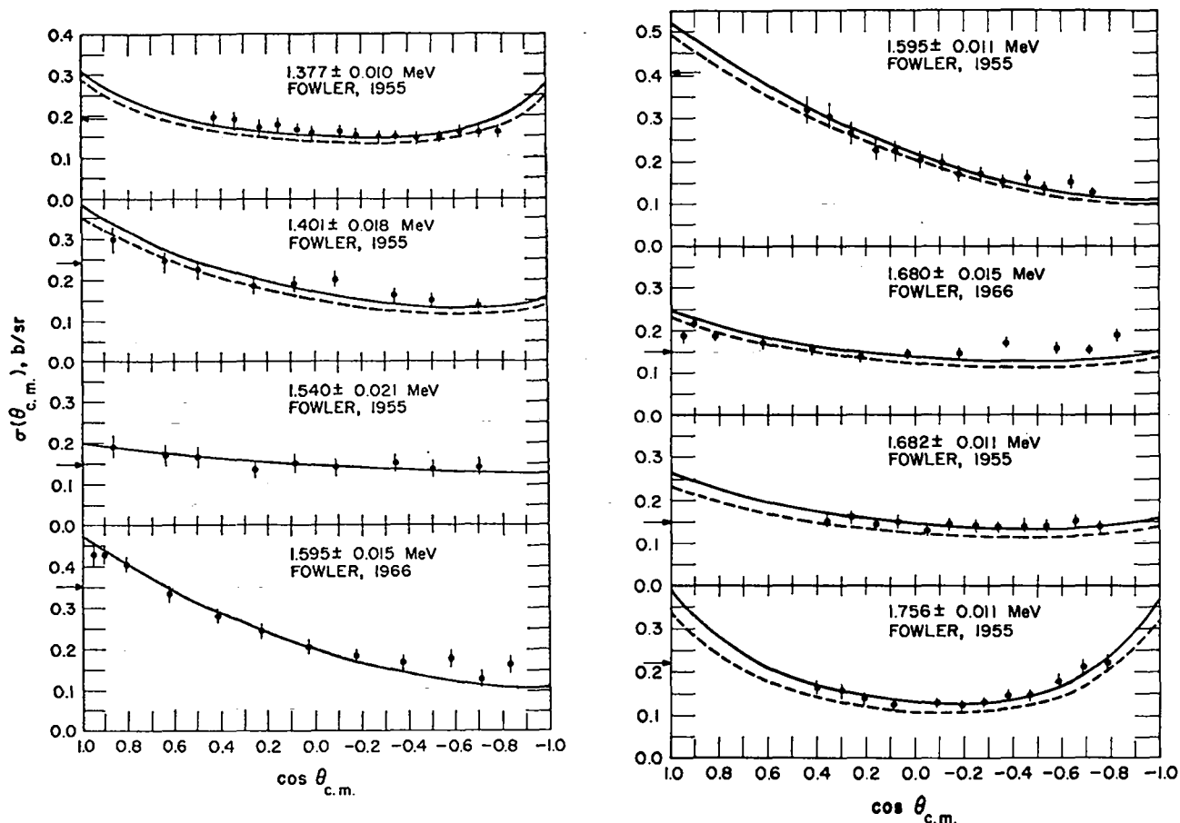
Fig. 75. Measured and evaluated differential cross sections for elastic scattering from 1.37 to 1.76 MeV.
