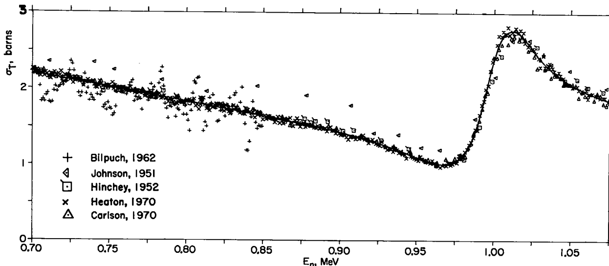
Fig. 9. Measured and evaluated total cross section between 0.7 and 1.1 MeV.
