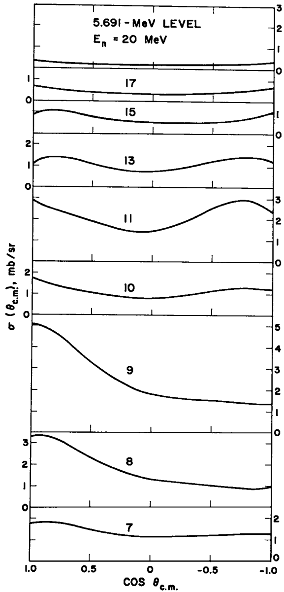
Fig. C10. Evaluated differential cross sections at selected energies for inelastic scattering to the 5.691-MeV level in 14 N.
