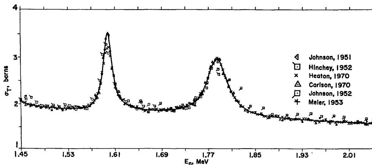
Fig. 11. Measured and evaluated total cross section between 1.45 and 2.05 MeV.
