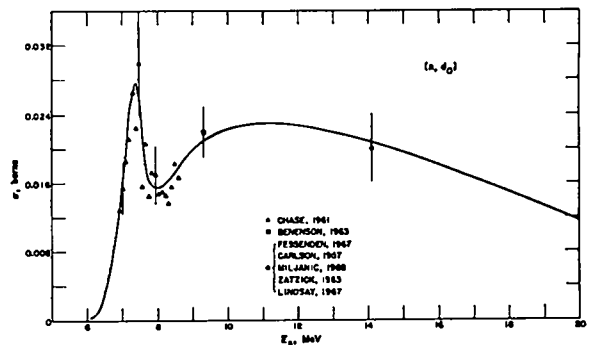
Fig. 48. Measured and evaluated (n,d) cross sections to the ground state of ^{13}\text{C} . The 14-MeV point is a composite of five measurements.
