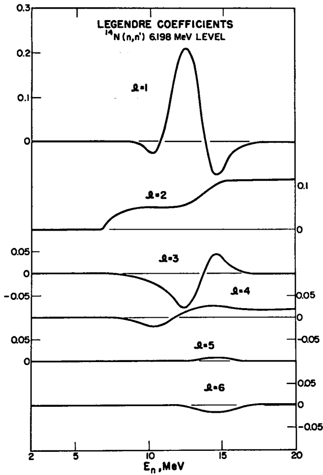
Fig. C13. Evaluated Legendre coefficients for inelastic scattering to the 6.198-MeV level in 14 N.
