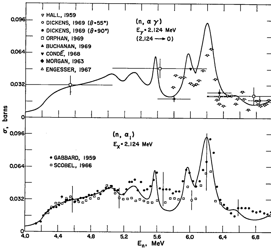
Fig. 59. Measured and evaluated (n, \alpha_1) and (n, \alpha \gamma) cross sections for the 2.124-MeV level and ground-state transition for neutron energies between 4 and 7 MeV.
