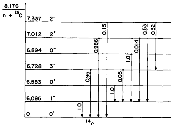
Fig. 45. Decay scheme for ^{14}\text{C} used in correlating the (n,p\gamma) cross sections with the level-excitation cross sections. Note that the energy scale is grossly distorted.
