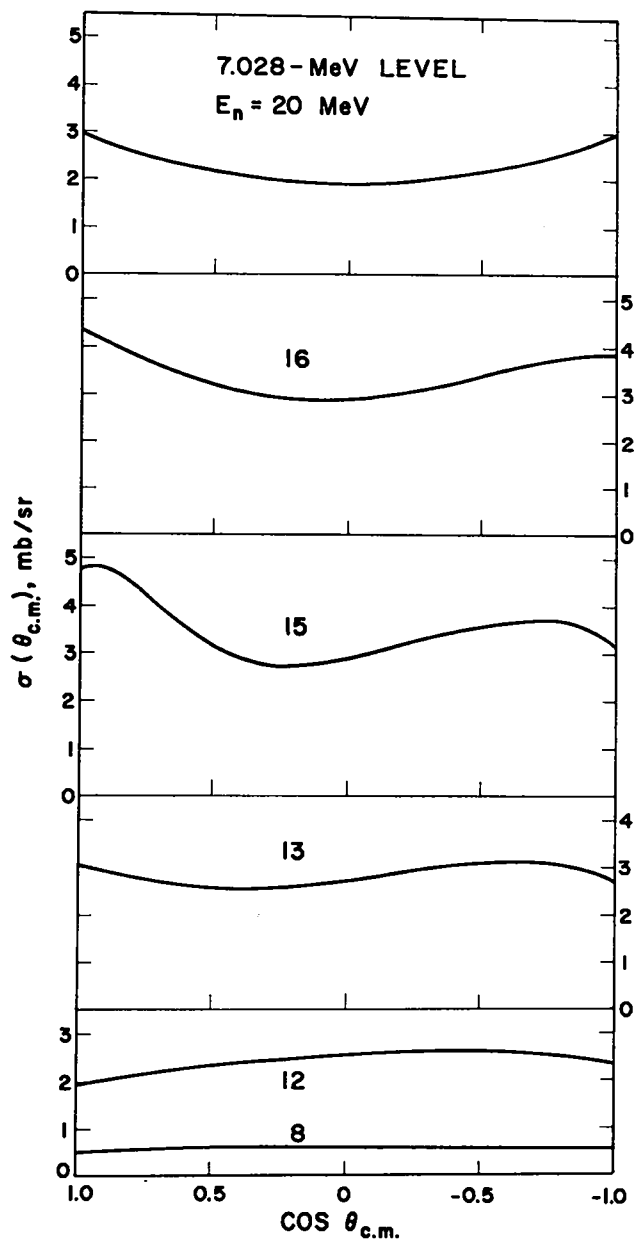
Fig. C18. Evaluated differential cross sections at selected energies for inelastic scattering to the 7.028-MeV level in 14 N.
