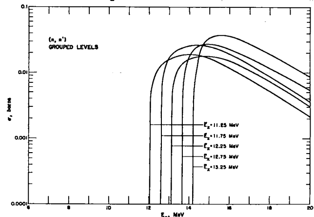
Fig. 37. Evaluated (n,n') cross sections to groups of levels in ^{14}\text{N} between 11 and 13.5 MeV.
