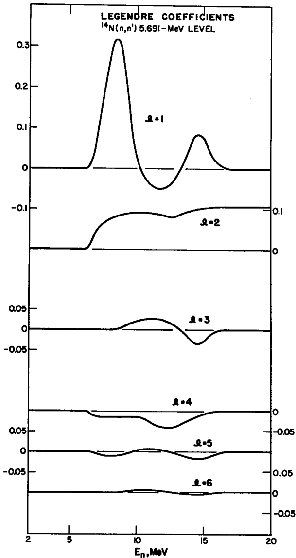
Fig. C9. Evaluated Legendre coefficients for inelastic scattering to the 5.691-MeV level in 14 N.
