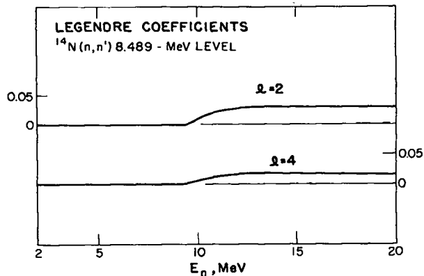
Fig. C23. Evaluated Legendre coefficients for inelastic scattering to the 8.489-MeV level in ^{14}\text{N} , assumed symmetric in the absence of adequate data.
