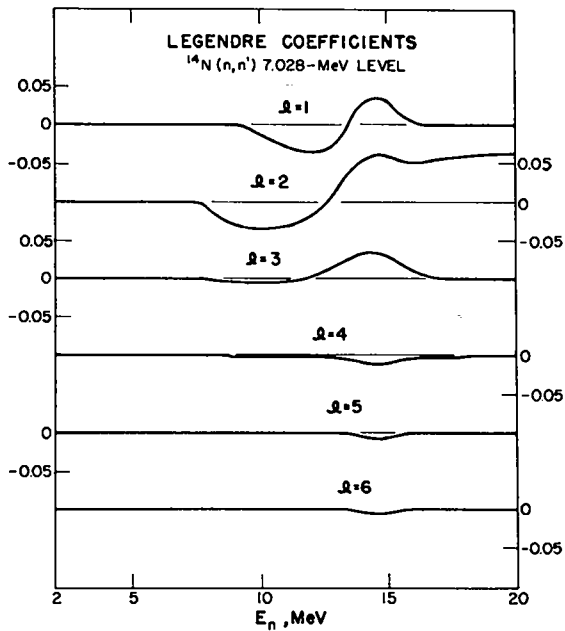
Fig. C17. Evaluated Legendre coefficients for inelastic scattering to the 7.028-MeV level in 14 N.
