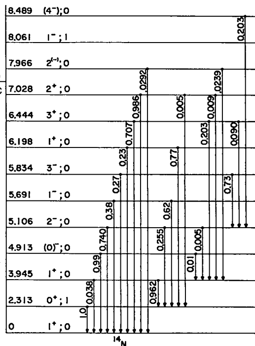
Fig. 23. Decay scheme for ^{14}\text{N} used in interpreting the (n,n'\gamma) measurements. The levels are labeled with their isospin as well as ordinary spin and parity. Note that the energy scale is distorted.
